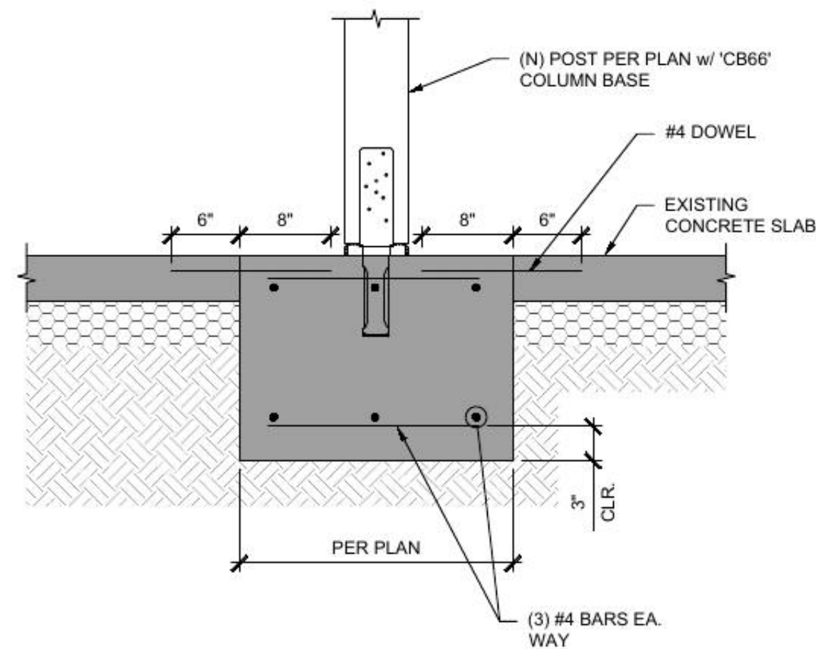
1 (N) FOOTING & POST AT (E) FOOTING SCALE: 1"=1'-0"
