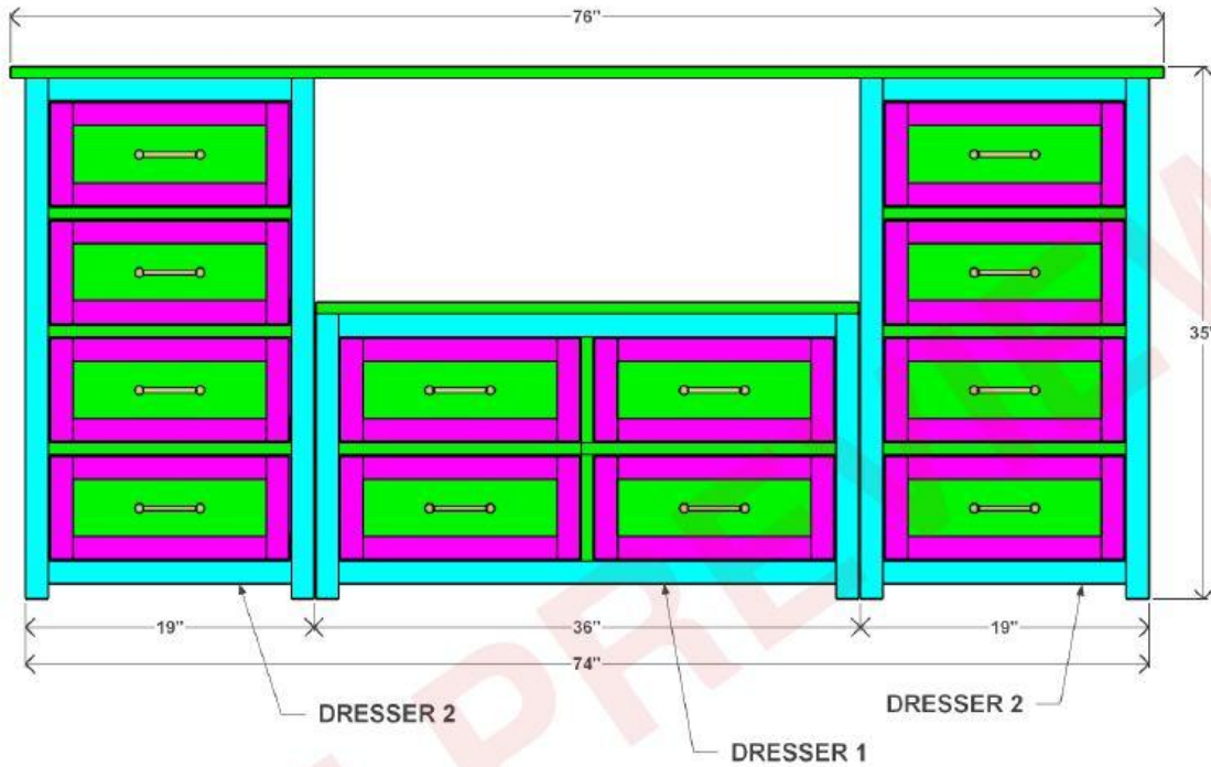
FRONT VIEW
