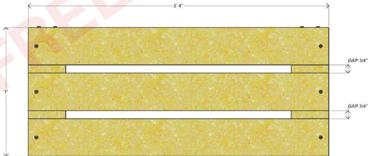
TOP VIEW
