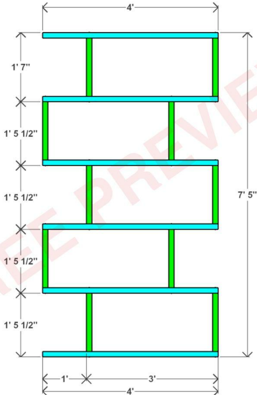
FRONT VIEW
