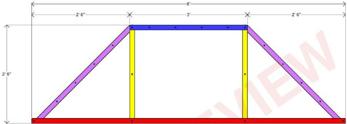
FRONT VIEW
