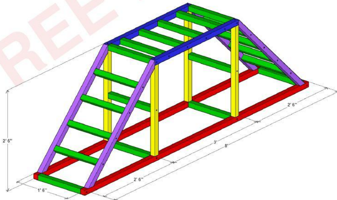
3D VIEW
