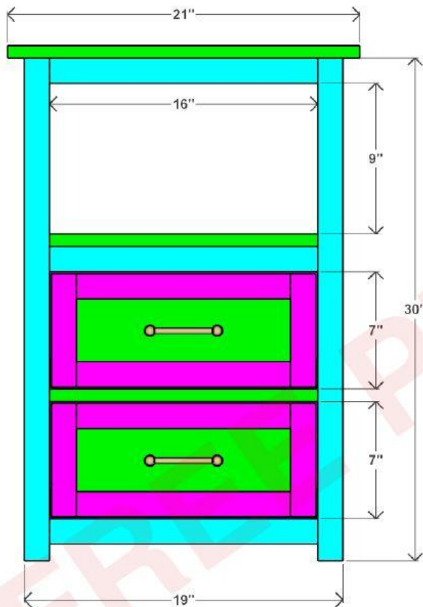
FRONT VIEW
