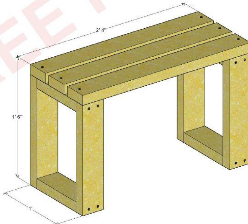
3D VIEW
