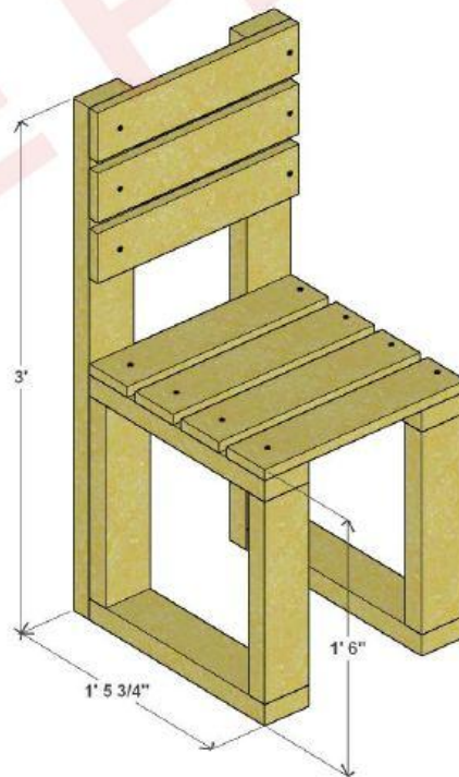
CHAIRS 3D VIEW
