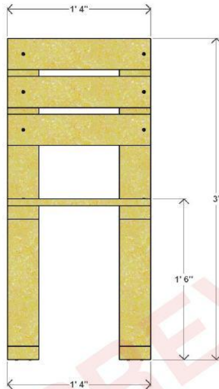
CHAIRS FRONT VIEW
