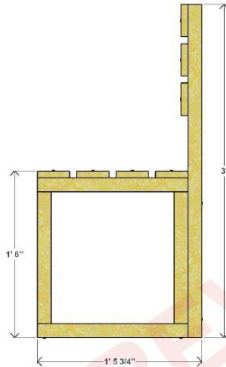
CHAIRS SIDE VIEW
