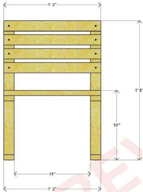
CHAIR FRONT VIEW
