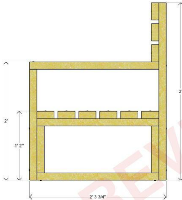
THREE SEATER CHAIR SIDE VIEW
