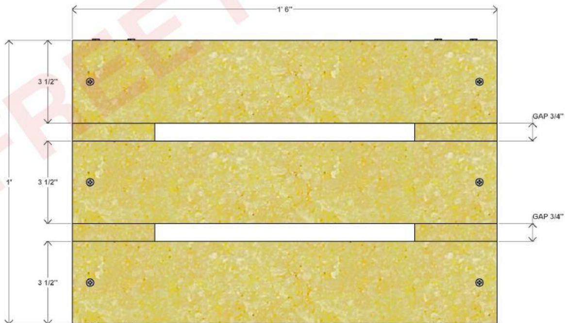
TOP VIEW
