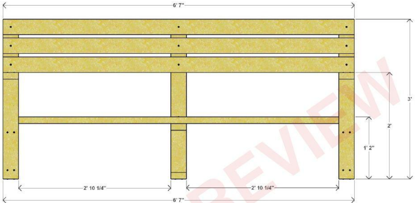
THREE SEATER CHAIR FRONT VIEW
