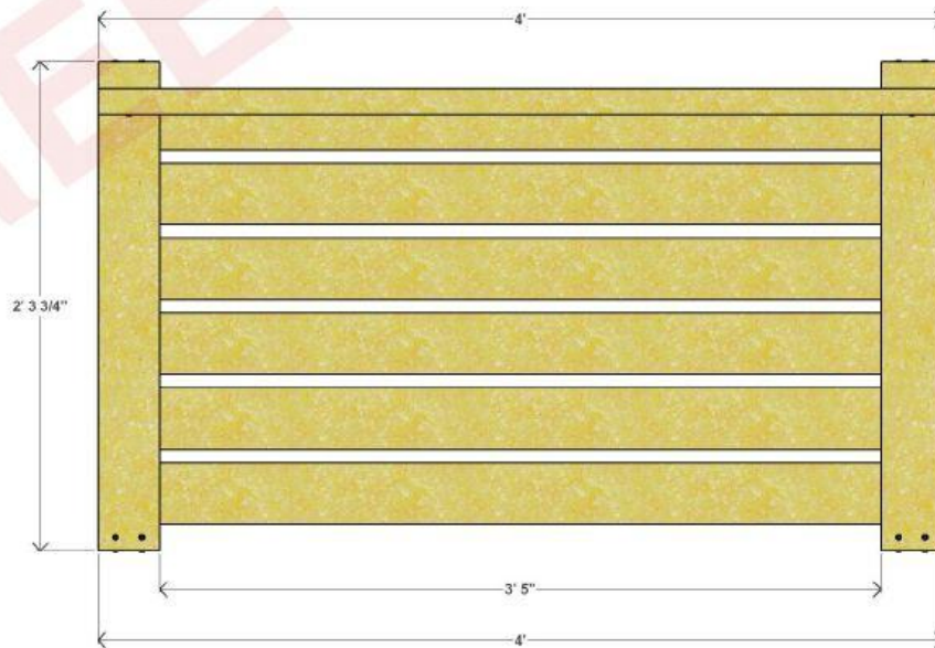
CHAIR TOP VIEW
