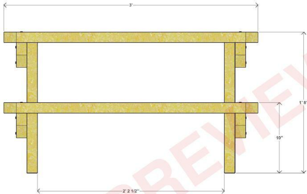
FRONT VIEW
