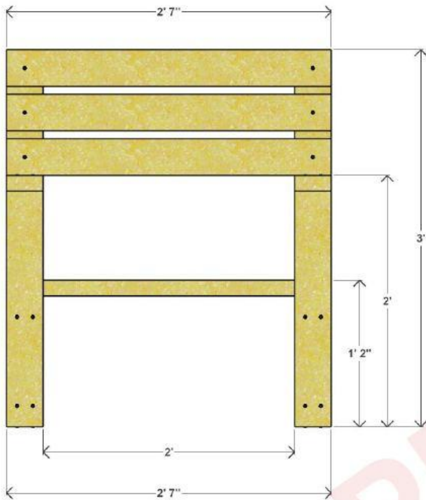
CHAIR FRONT VIEW
