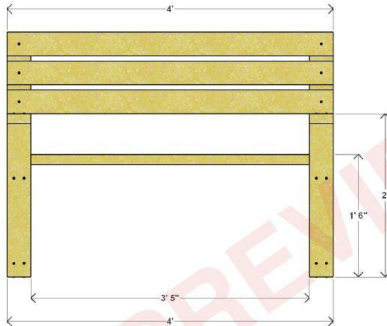
CHAIR FRONT VIEW
