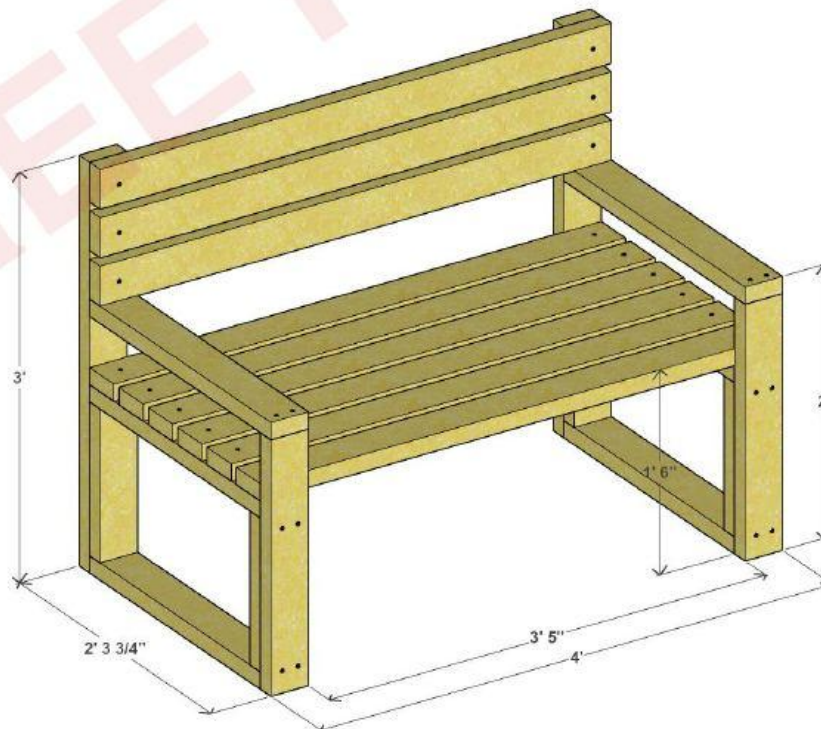
CHAIR 3D VIEW
