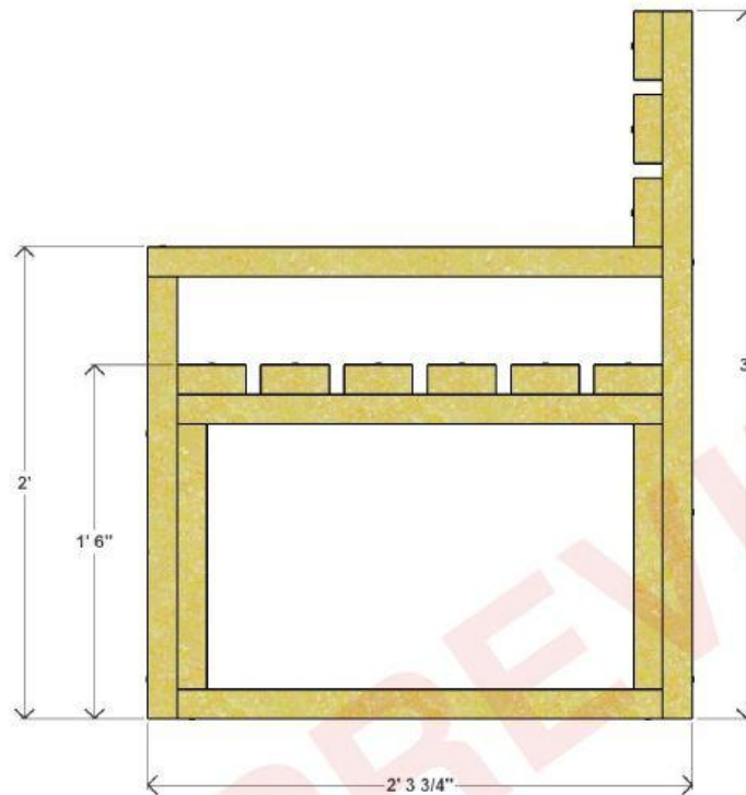
CHAIR SIDE VIEW
