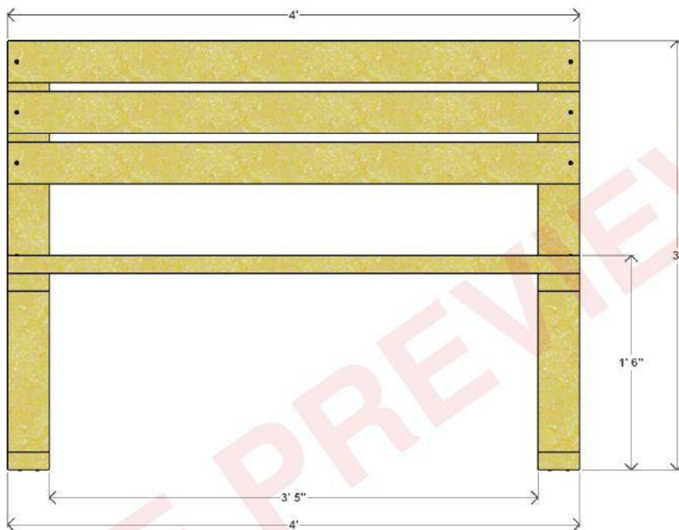
FRONT VIEW
