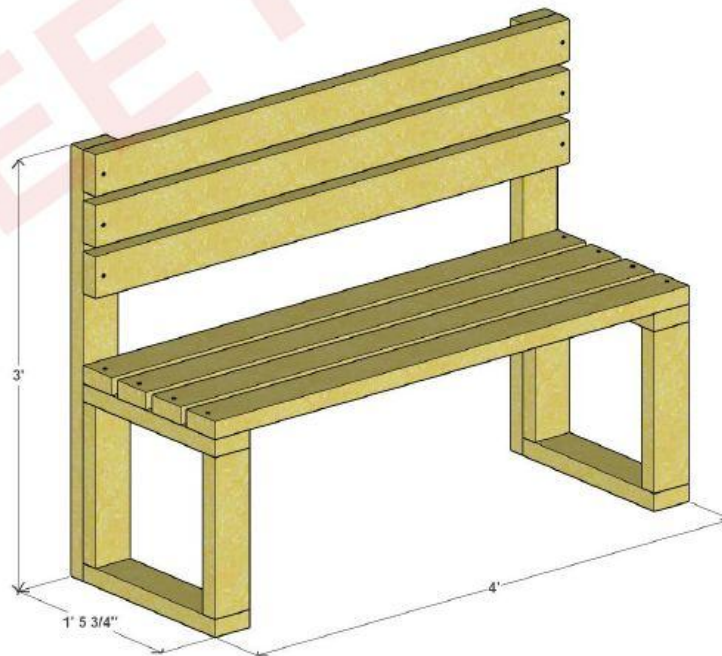
3D VIEW
