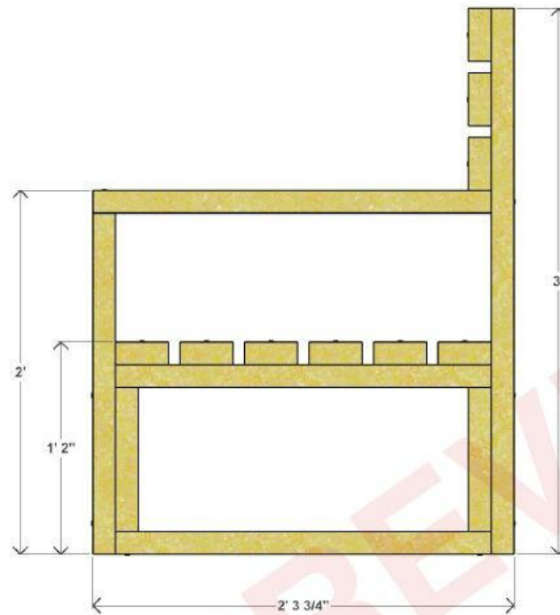
TWO SEATER CHAIR SIDE VIEW
