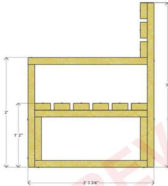
ONE SEATER CHAIR SIDE VIEW
