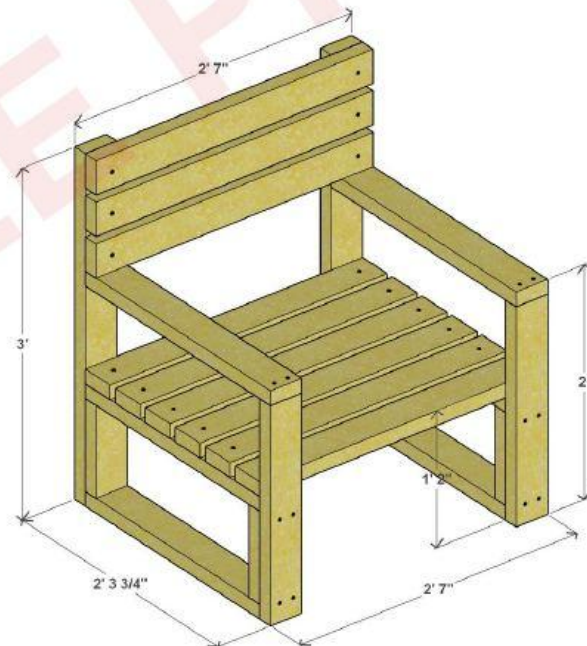
ONE SEATER CHAIR 3D VIEW
