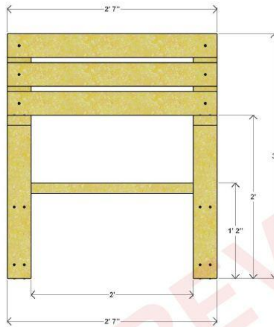
ONE SEATER CHAIR FRONT VIEW
