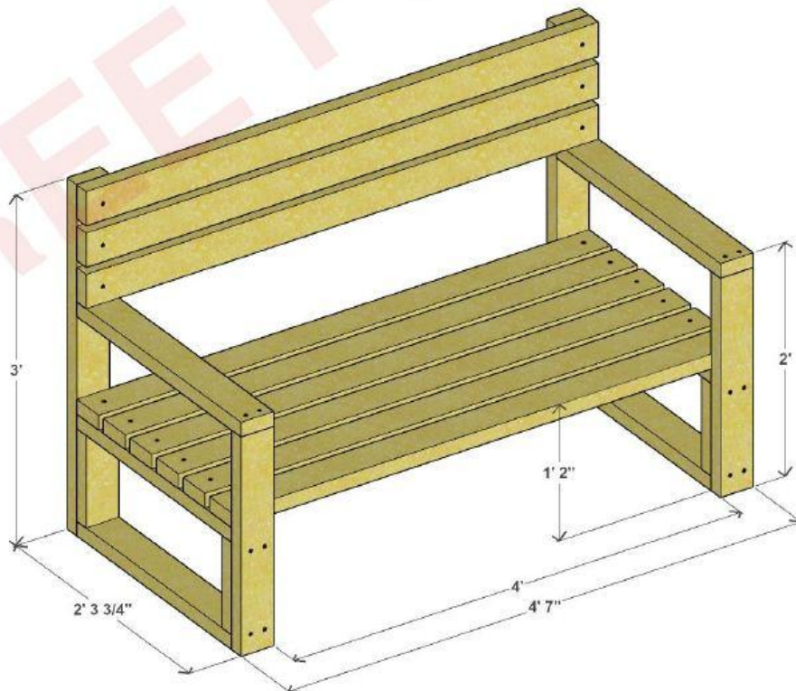
TWO SEATER CHAIR 3D VIEW
