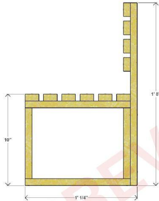
CHAIR SIDE VIEW
