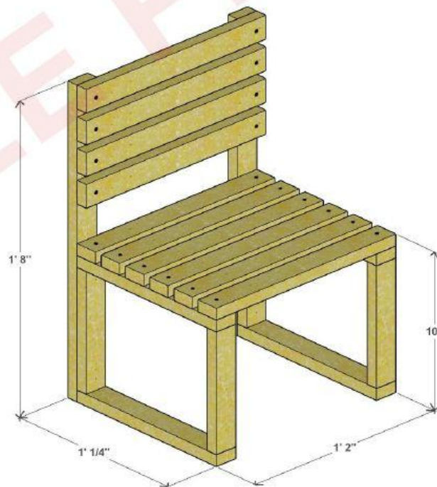
CHAIR 3D VIEW
