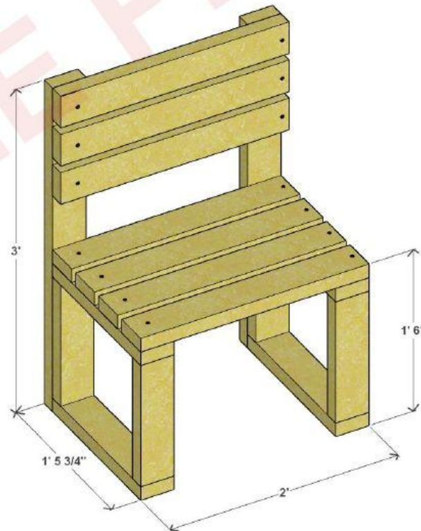
3D VIEW
